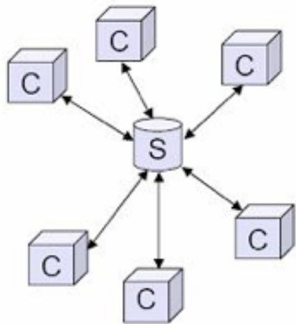
Client/Server
